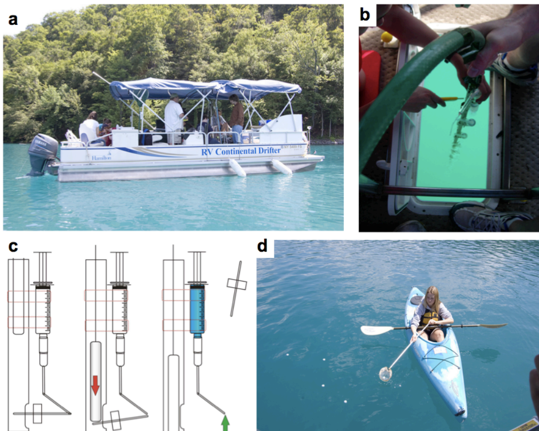
Figure 3: (a,b) Deployment and operation of the multilevel sampler. (c) Mechanism of sample collection. Sterile syringes are fitted with bent flame sealed glass Pasteur pipettes and deployed under vacuum. Each syringe is fitted with a numbered float. (d) Upon triggering, floats are collected to confirm water was collected at the target depth.
