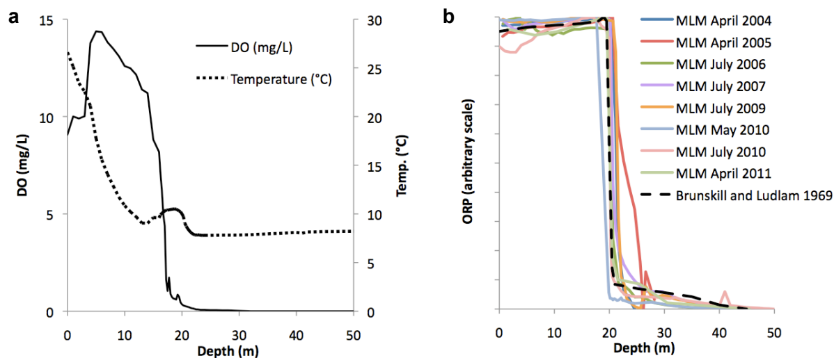
Figure 5: (a) Dissolved oxygen and temperature profiles in Green Lake for July 2008. The redoxcline was located at 20.5 meters. (b) Compilation of oxidation reduction potential measurements made between 2004 and 2011 compared to the measurement of Brunskill and Ludlam (1969).
