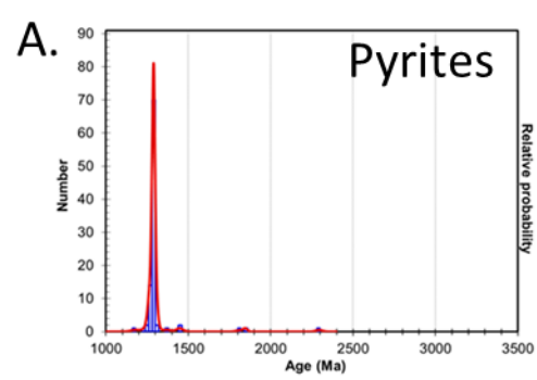
Figure 8. On left schematic cartoon showing the development and fill of the Trans-Adirondack Back-arc Basin. On the right, relative probability histograms for zircon populations from each stage of basin evolution. See text for detailed explanation. Note that in contrast to the quartzites from Pyrites and the Lower and Upper Marbles, the Popple Hill Gneiss is dominated by anatectic or metamorphic zircon formed during the height of Shawinigan metamorphism (ca. 1170 Ma). Detrital zircons yield ages mostly between 1300-1400 Ma (Heumann et al., 2008).
