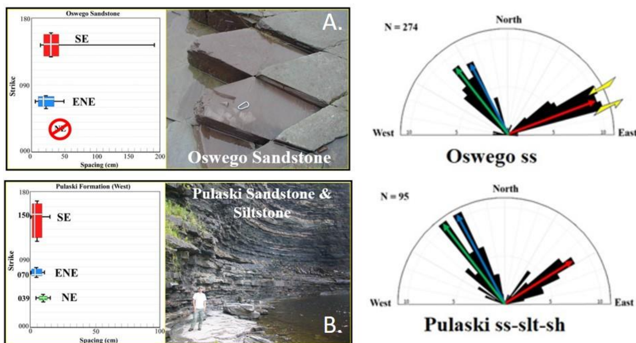
Figure 7. Box and whisker plots and rose diagrams showing the orientations and spacing of fracture sets in the Oswego (A) and Pulaski (B) Formations at Salmon River falls.
